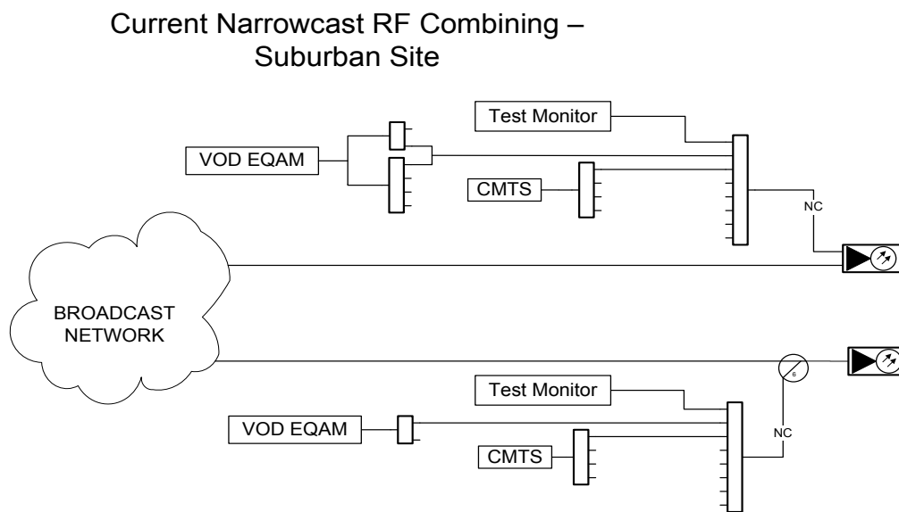
Figure 1a – RF Combining Example: Existing
