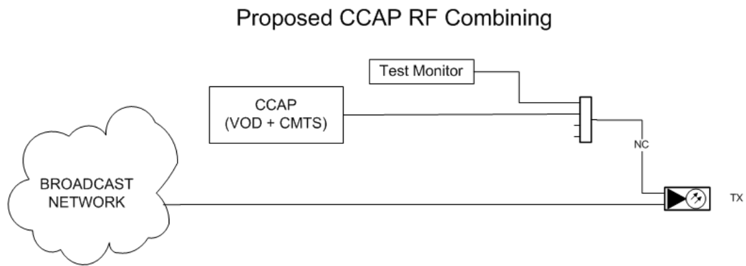
Figure 1b – RF Combining Example: After CCAP Migration
