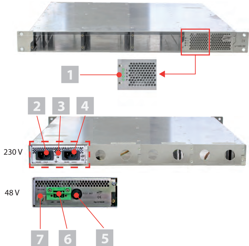
Figure 1: U 100 - base unit
