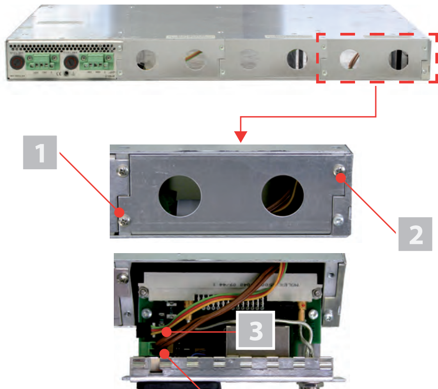
Figure 3: Installing the backplane in the base unit
