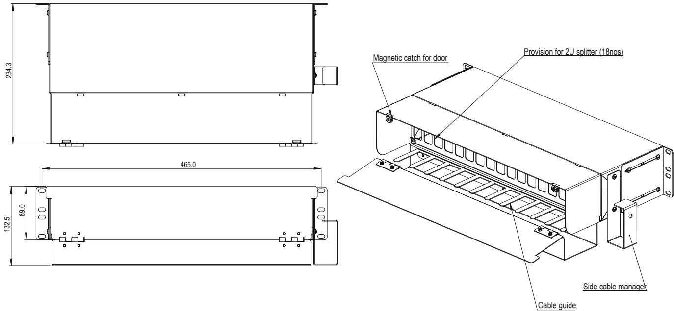
2U PLC GEN2 Splitter Chassis
